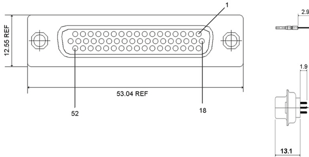
Figure 1: CON/KAD/004 front view
