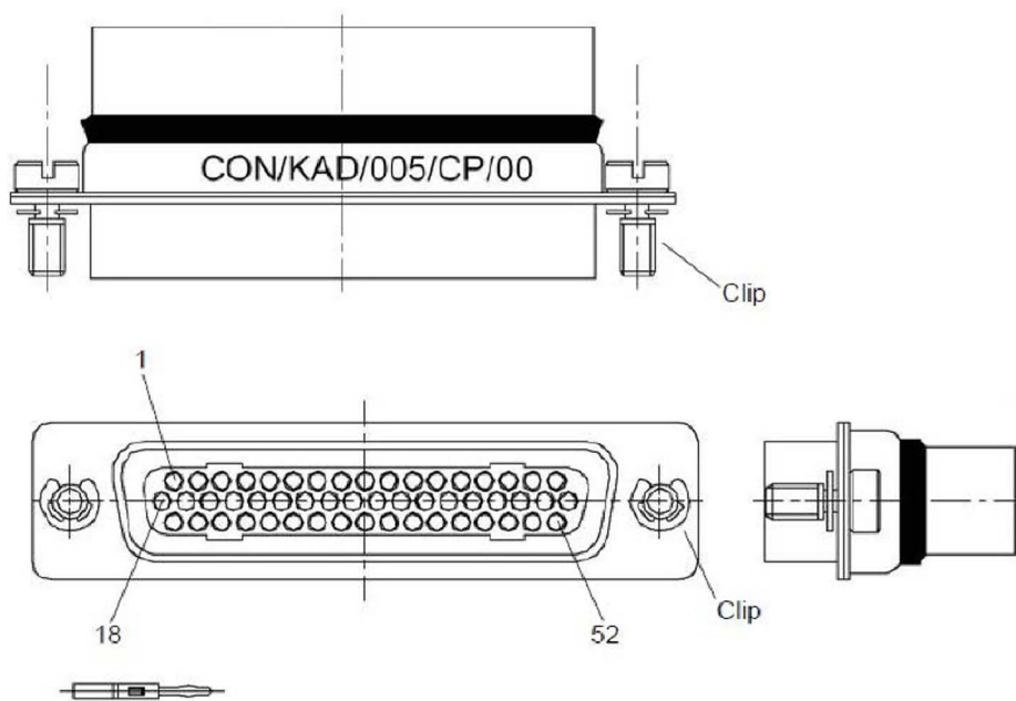
Figure 1: CON/KAD/005/CP plan, elevation and front view
