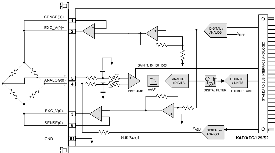
Figure 1: First of four channels on the KAD/ADC/129/S2
