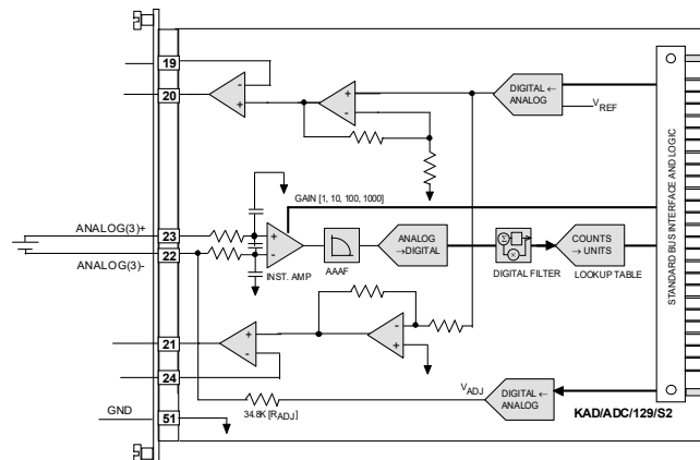
Figure 4: Fourth of 4 independent differential ended channels
