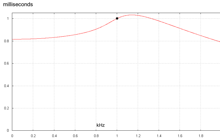
Figure 6: Filter delay for 8 th order Butterworth filter where f_c = 1\text{kHz}
