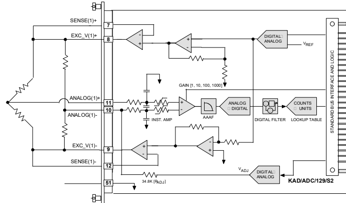
Figure 2: Second of 4 independent 1/2-bridge channels with matched pair completion resistors
