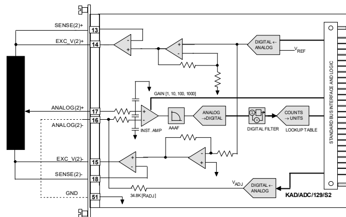
Figure 3: Third of 4 independent potentiometer channels
