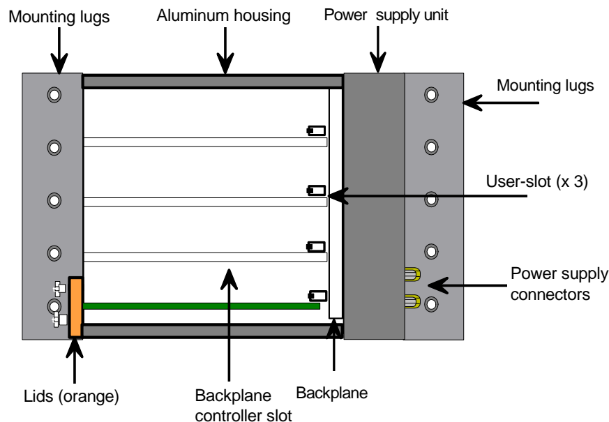
Figure 1: KAM/CHS/03F with PSU and three user-slots
