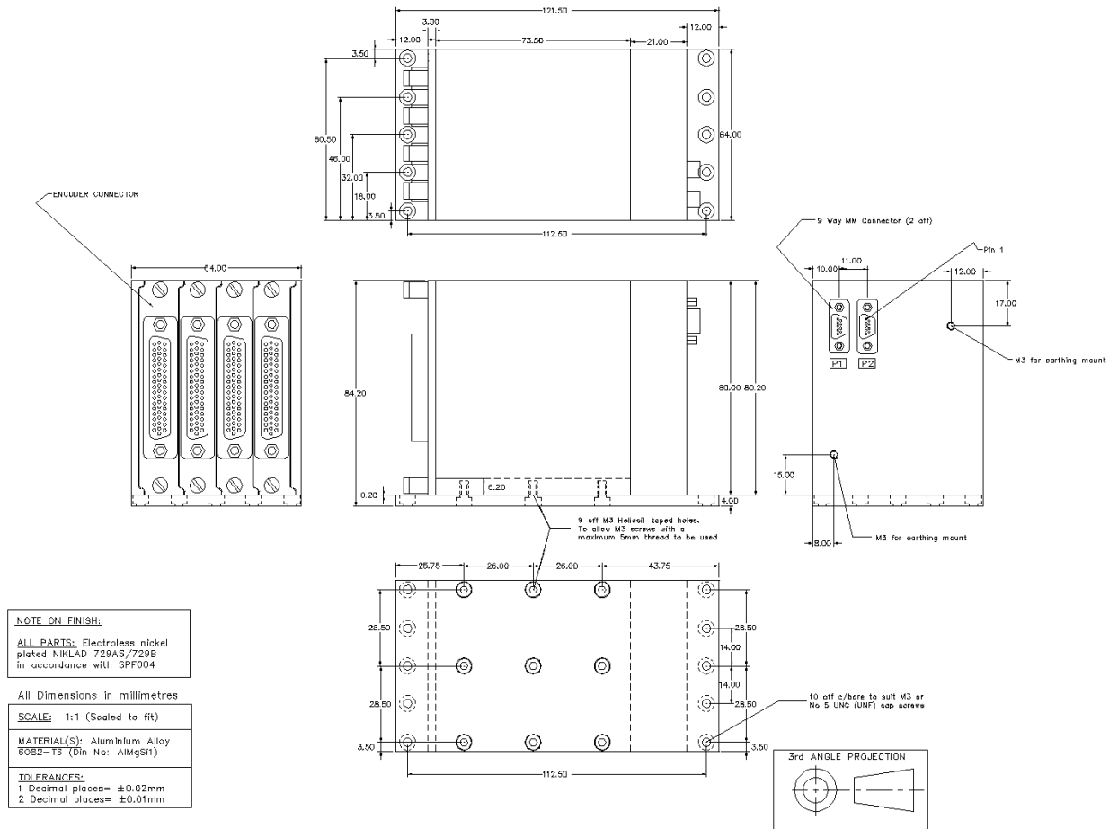
Figure 2: KAM/CHS/03F mechanical drawing
