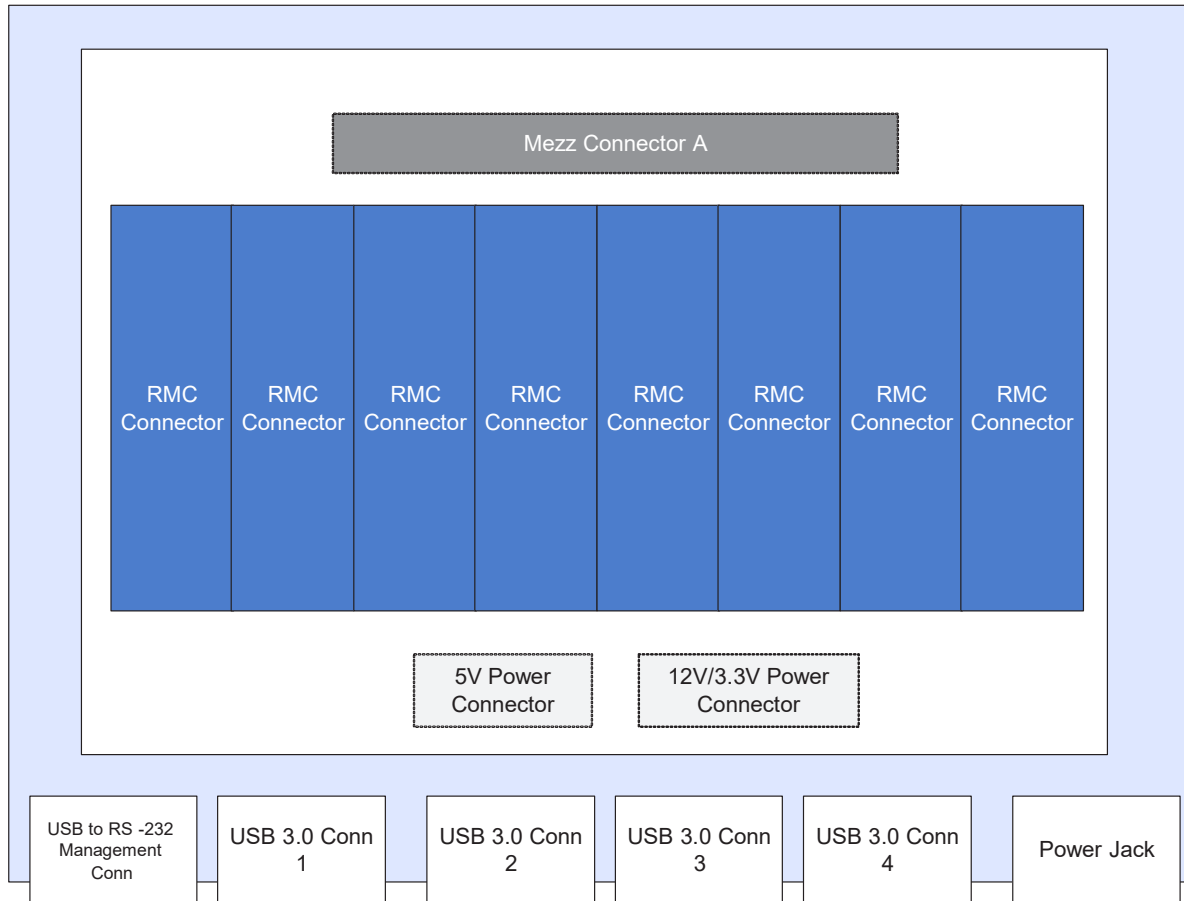
Figure 2: The docking station supports eight RMC.
