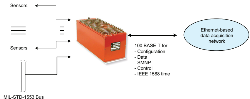
nDAU-2010/12/16 Functional block diagram
