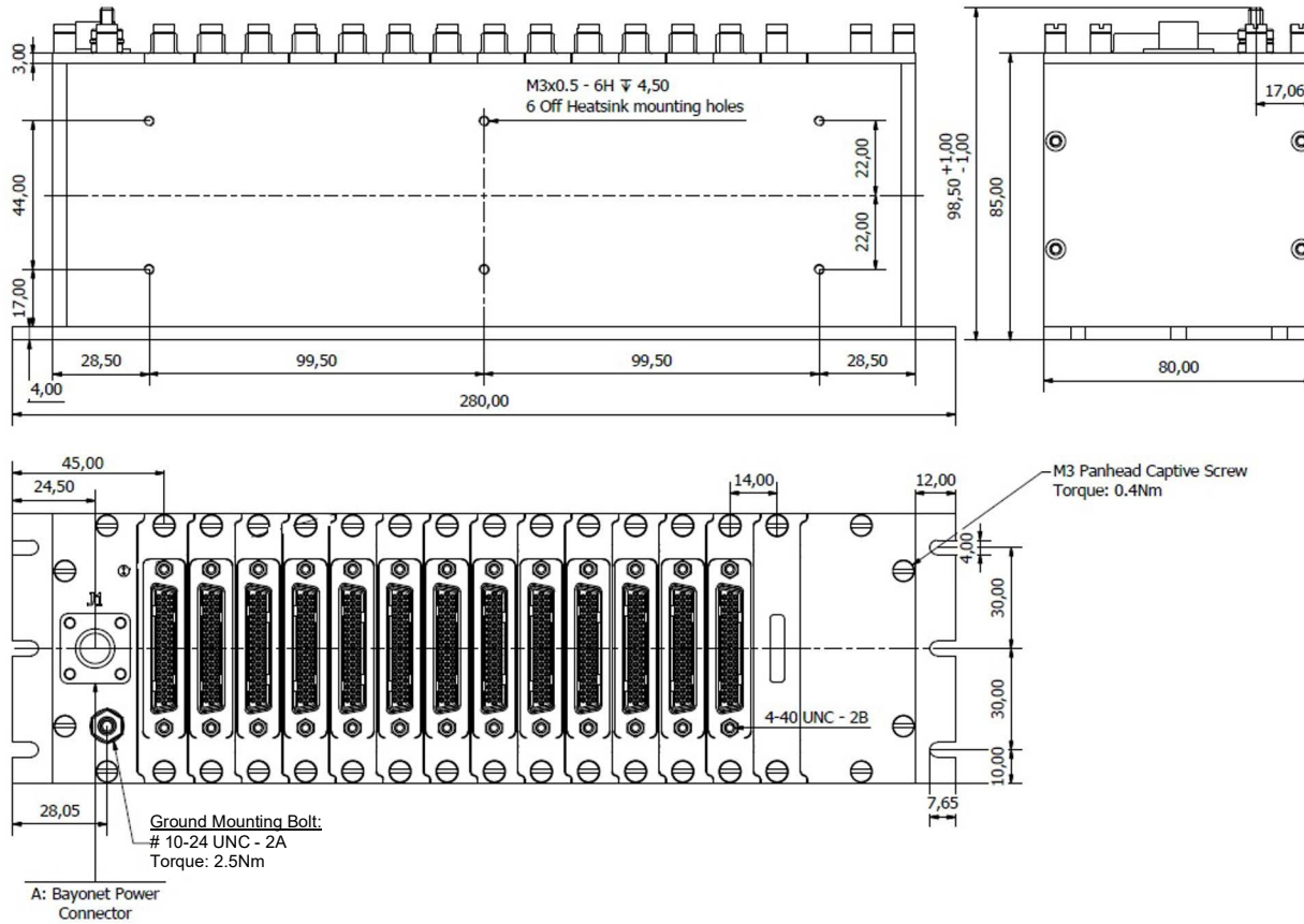
Figure 2: KAM/CHS/13U mechanical drawing
