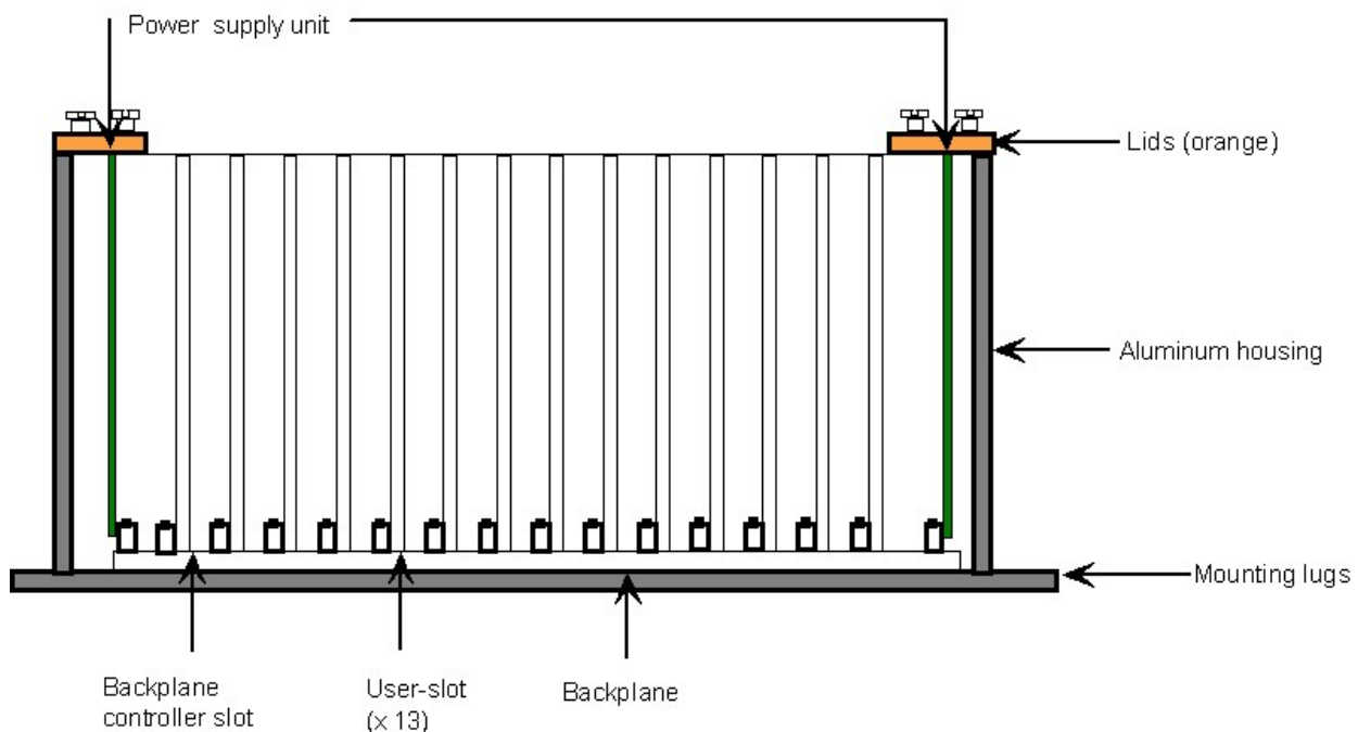
Figure 1: KAM/CHS/13U with PSU and thirteen user-slots
